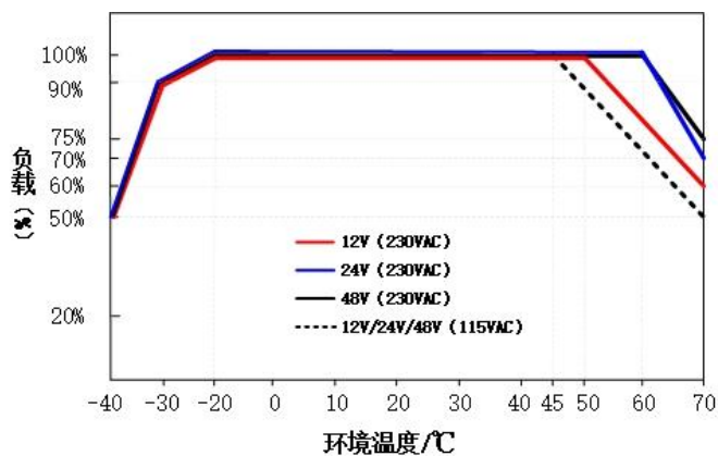
■ 降额曲线 Derating Curve
